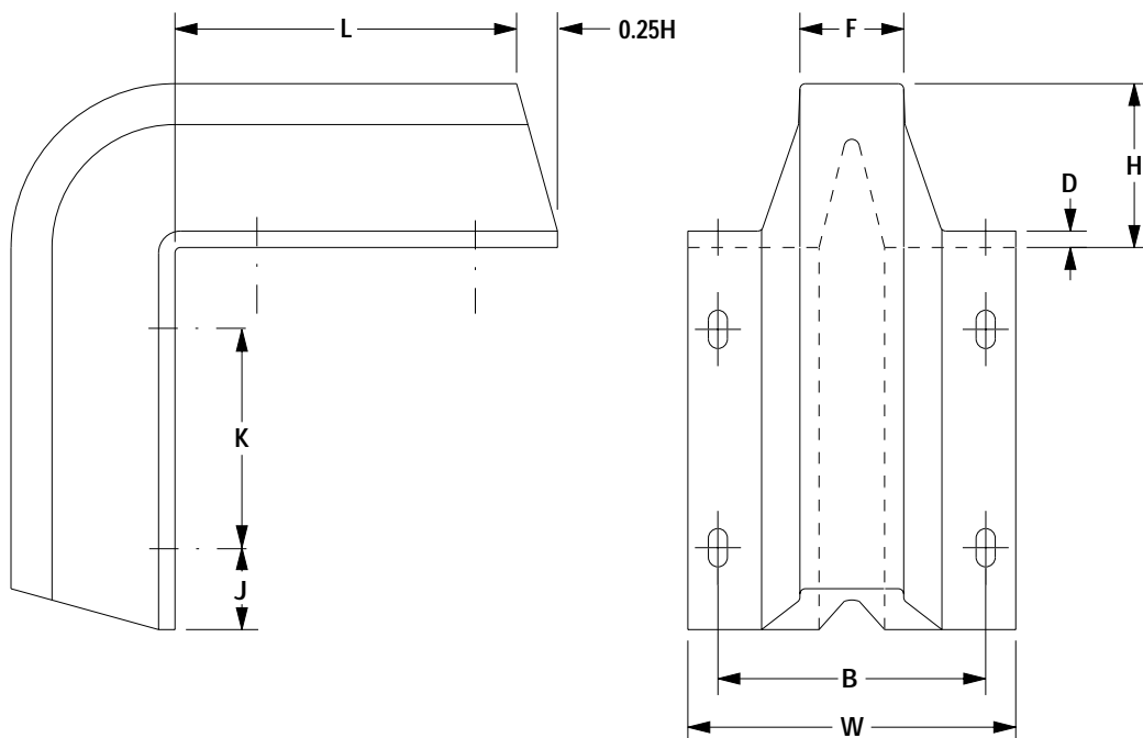
CORNER ARCH FENDER DIMENSIONS
