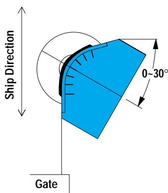
At the 90° entrance of a lock or dry dock
