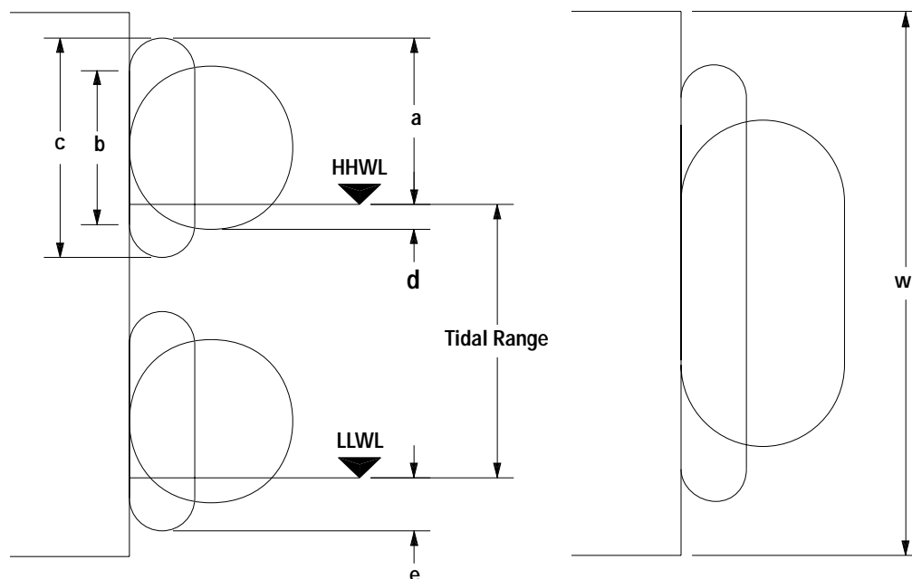
FOAM FENDER INSTALLATION DIMENSIONS
