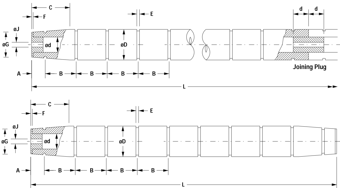
TUG CYLINDRICAL FENDERS
