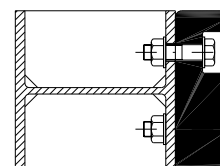
Fixing to steel columns
