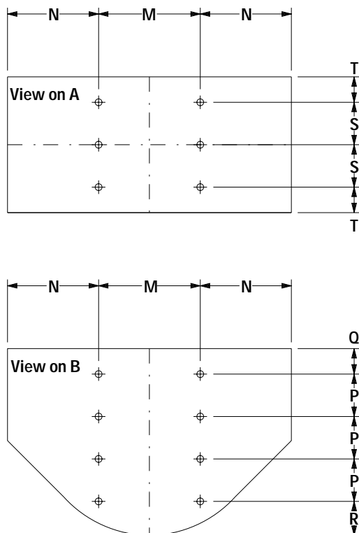
WHEEL FENDER ANCHOR LOCATIONS
