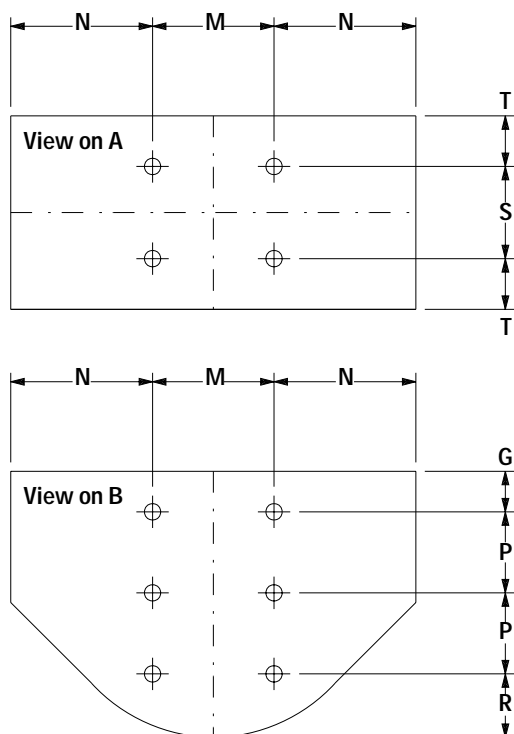
WHEEL FENDER ANCHOR LOCATIONS
