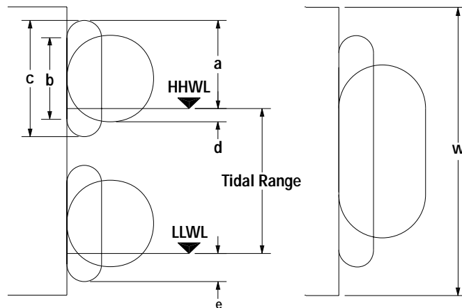
PNEUMATIC FENDER INSTALLATION DIMENSIONS
