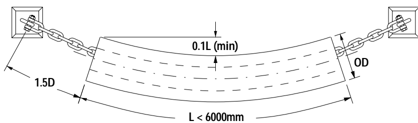
▲ Small cylindrical suspended with chain
