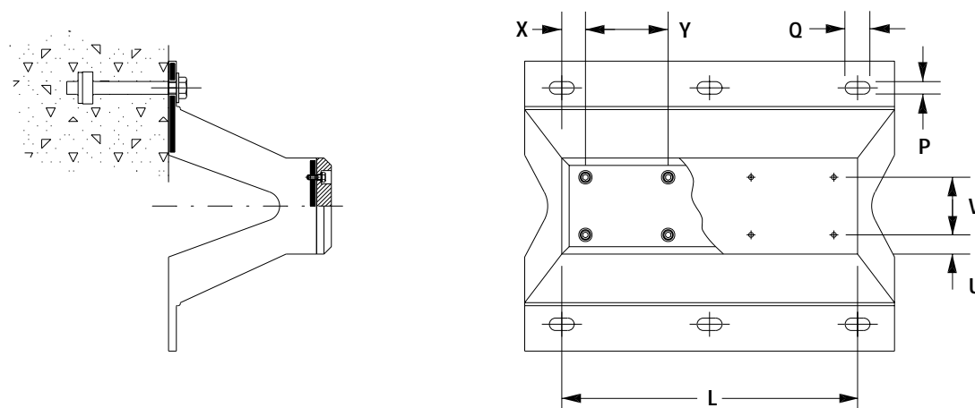
ANP ARCH FENDER
